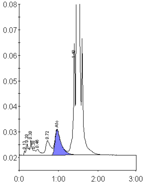
Peak table - ID: 10534133
